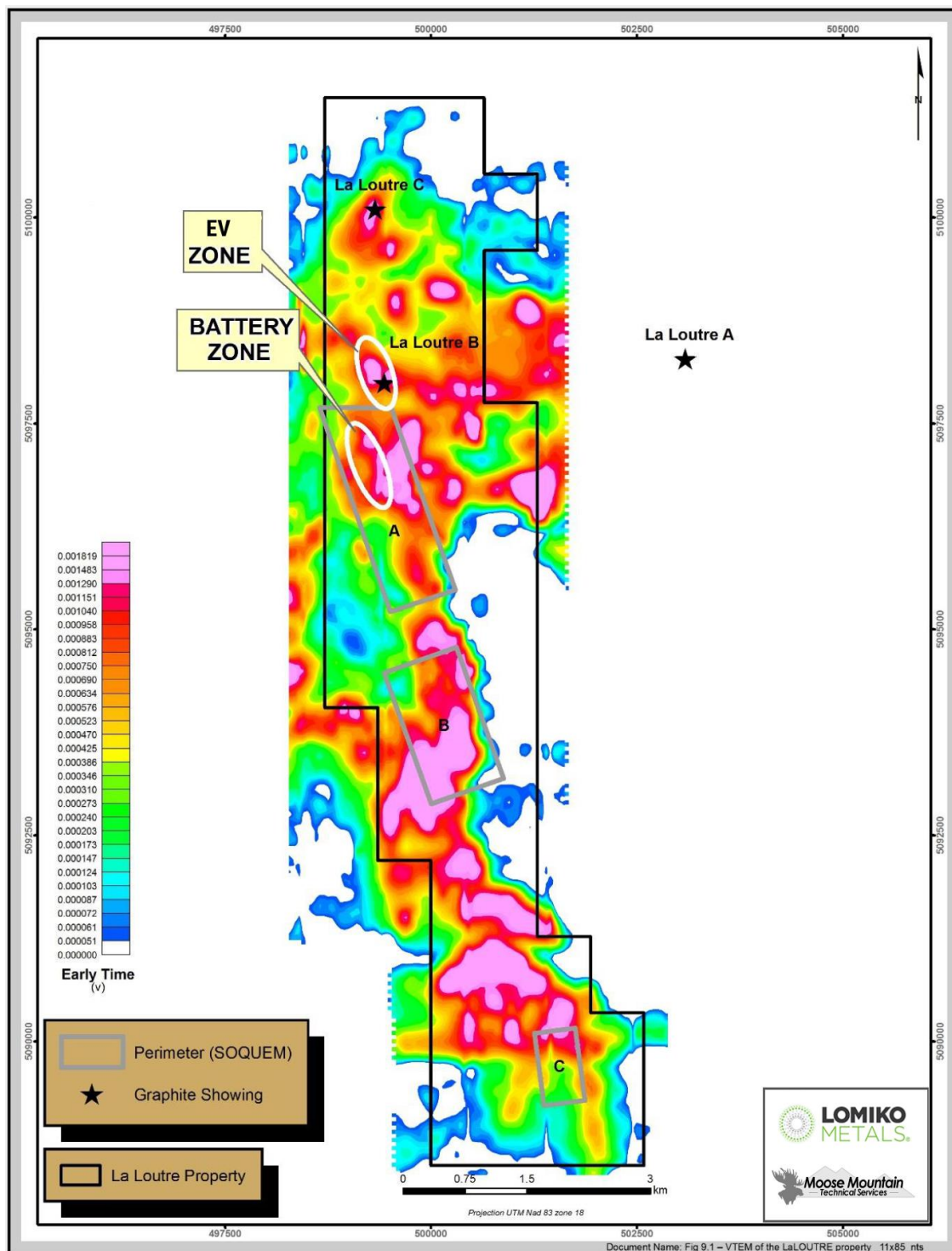
Figure 9-1: Map of the 2012 TDEM Survey (Early-Time EM Anomalies)
