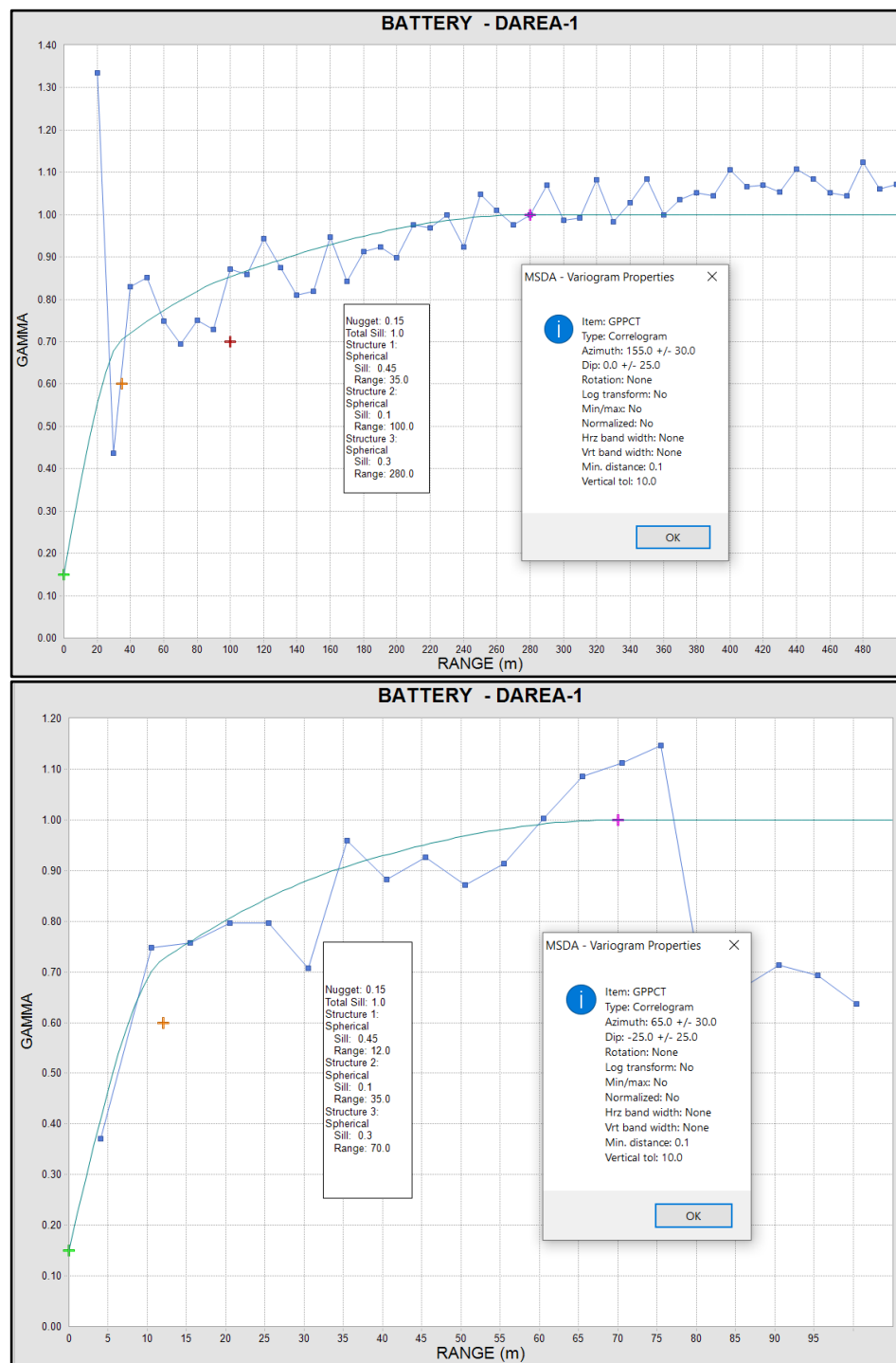
Figure 14-3: Battery Variography – Area 1 Major and Minor Axes
