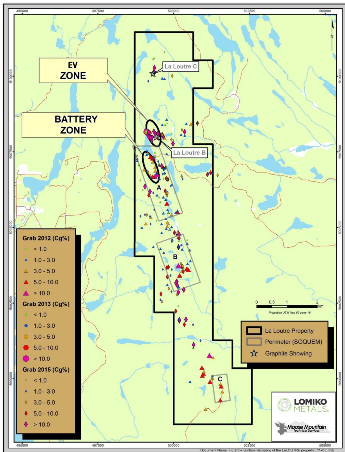
Figure 9-3: Grab Samples Collected by Consul-Teck on the La Loutre Property between 2012 and 2015
