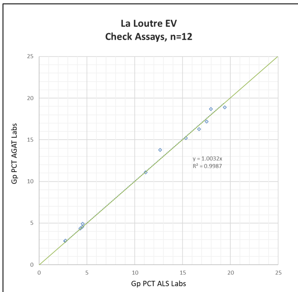
Figure 12-2: 2016 Check Assays, EV
