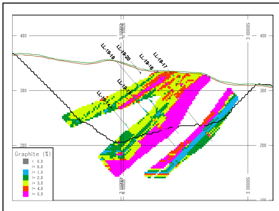
Figure 14-17: EV – Section E-E' – Drill Holes \pm 50 m
