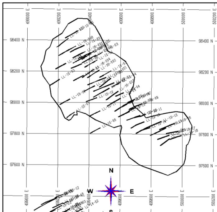
Figure 10-2: Collar Locations of Drill Holes in the EV Deposit
