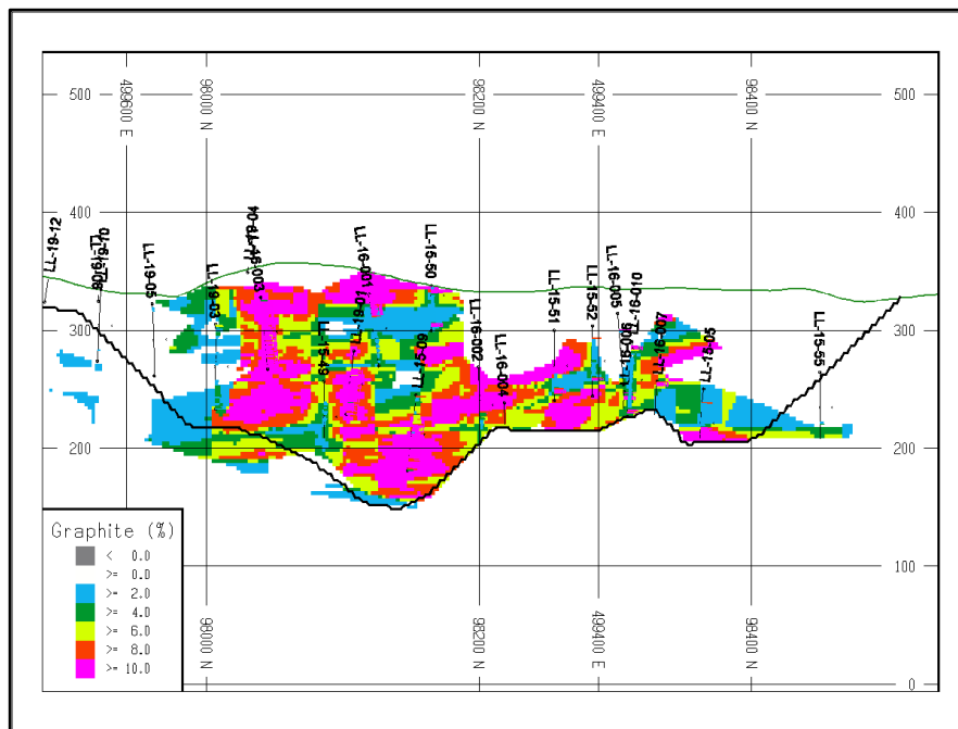
Figure 14-16: EV – Long Section D-D' – Drill Holes \pm 25 m
