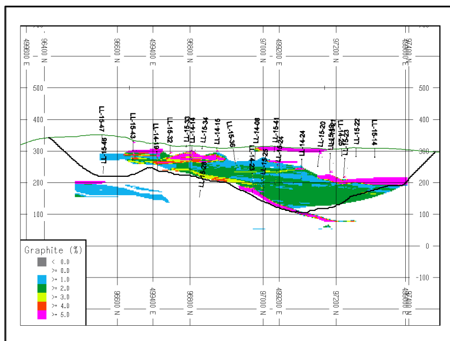
Figure 14-13: Long Section A-A' – Battery – Drill Holes \pm 25 m
